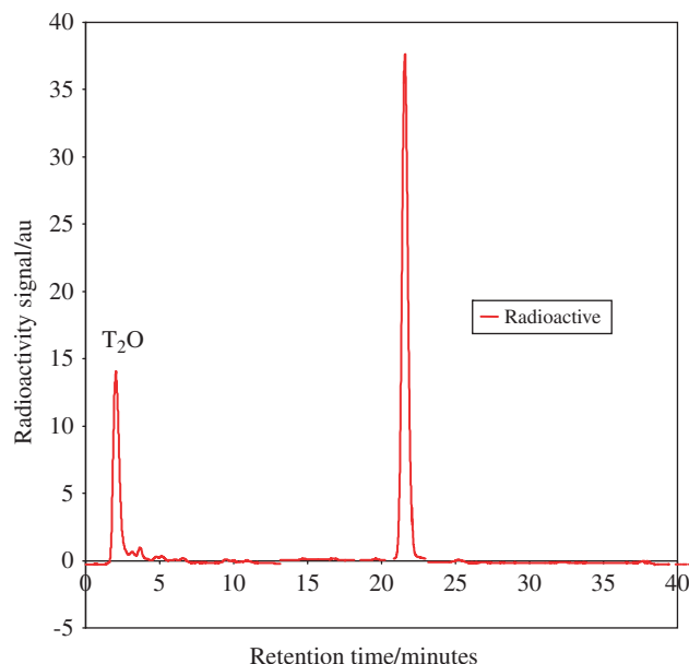
Figure 7. Radiochromatogram from the crude reaction mixture following a tritiation with complex 4c (5 mol%).
