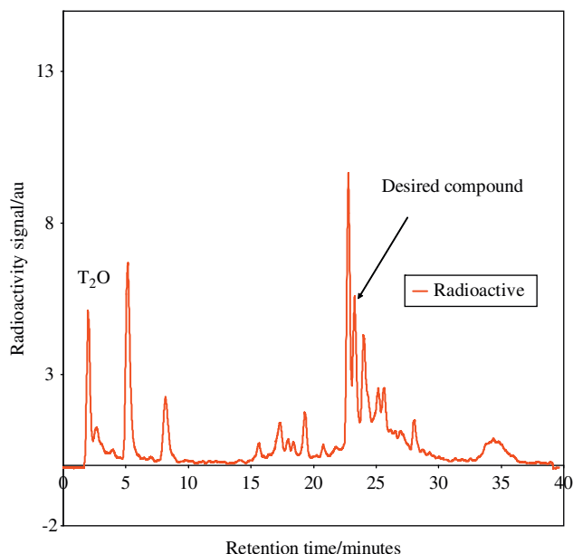
Figure 6. Radiochromatogram from the crude reaction mixture following a tritiation with Crabtree's catalyst (100 mol%).
