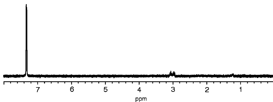
Figure 5. Tritium NMR of the tritiated product from the reaction of amide 5 with complex 4b (Scheme 5).
