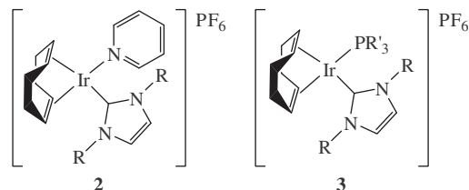
Figure 3. Modified iridium complexes possessing an NHC ligand.
